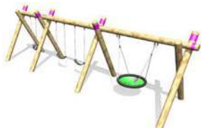
TAS3B 2x Belt, 1x Toddler, 1x Lillypad swings
