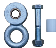
Clevis - Cast Type with M12 bush RP900 - Clevis RP906 - Bolt Set
