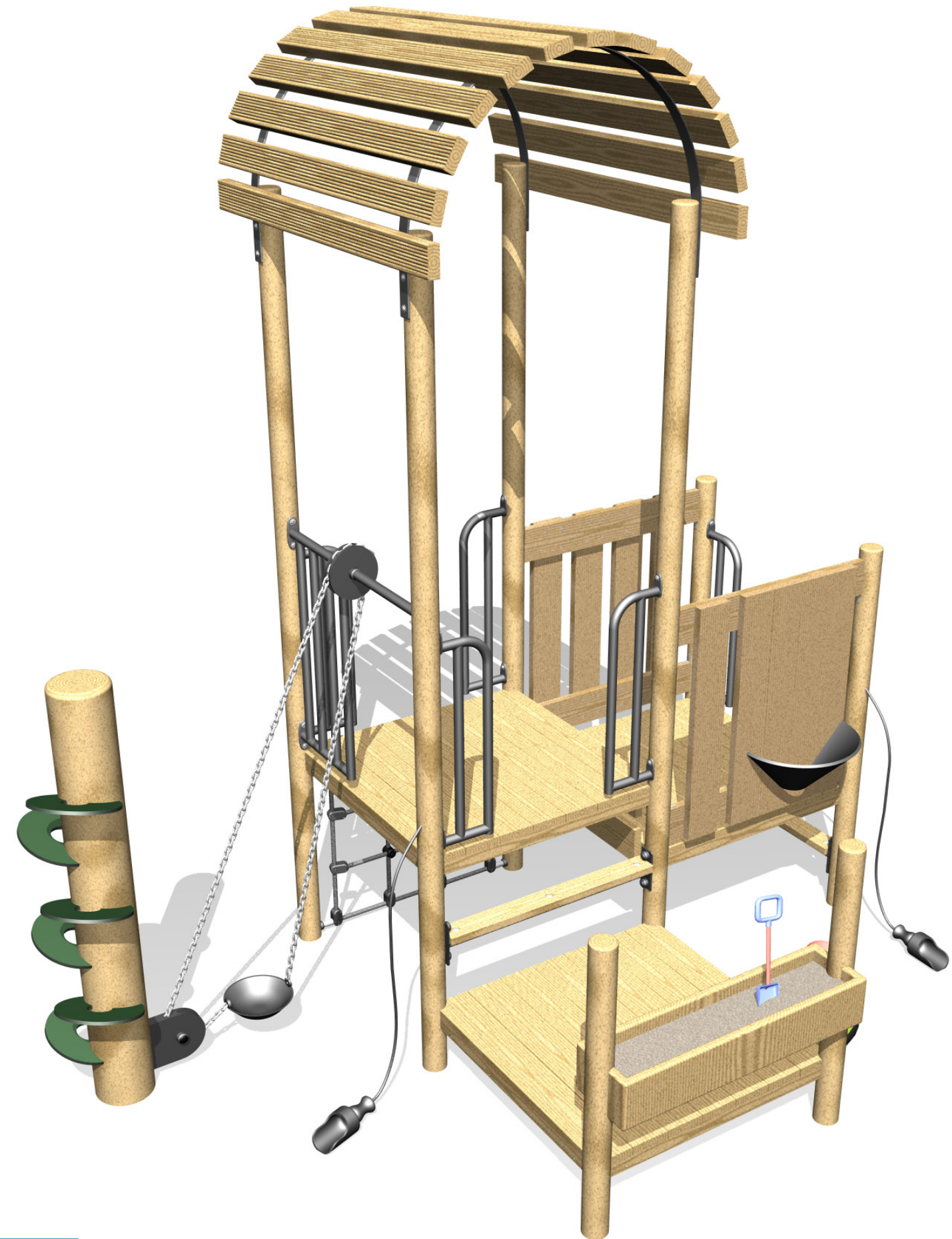
FS731 Sand play activity structure 01 2-12 6.2x5.2m 0.9m 2.3x3.3x3.5m Timber
